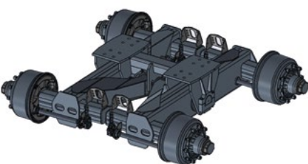
pendeltelg BPW
