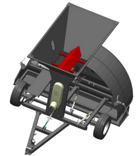
Slide to reduce pressure on the auger
