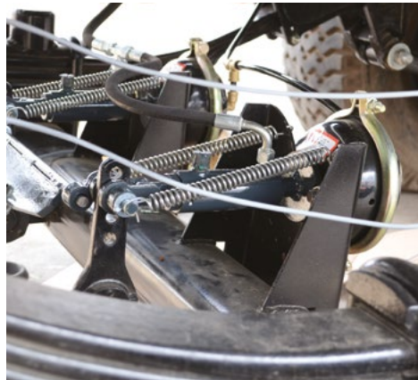
Combined braking system
